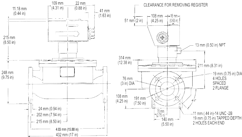
3" Type MP with 600 Series Register
