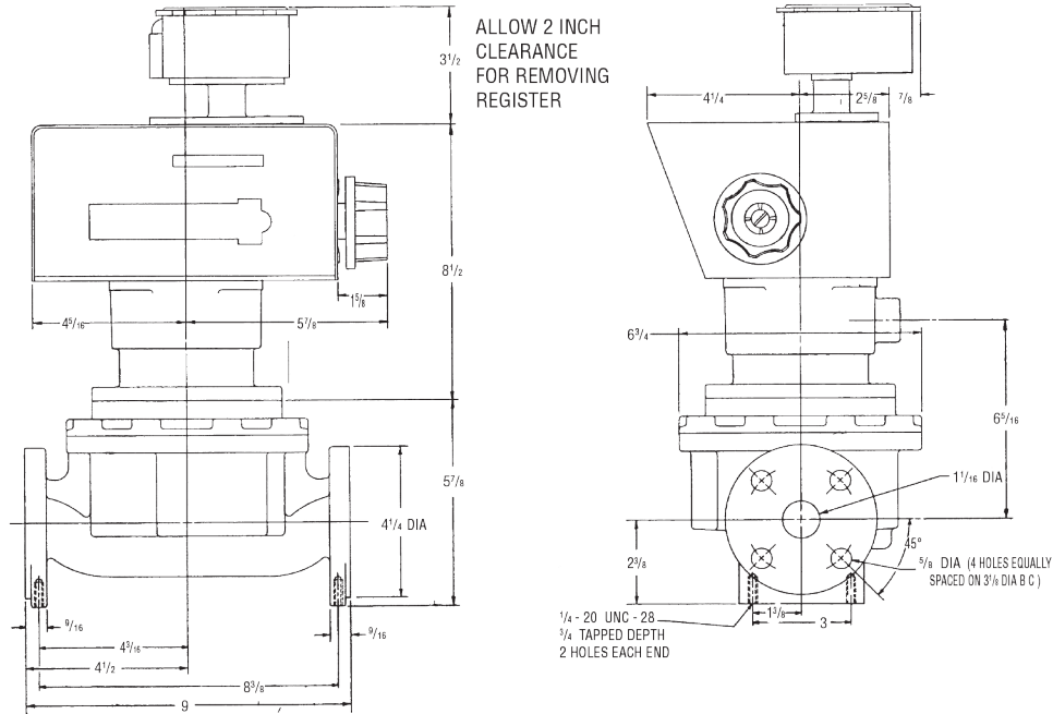
1" Type MP with 600 Series Register and Model 45 Pulse Transmitter
