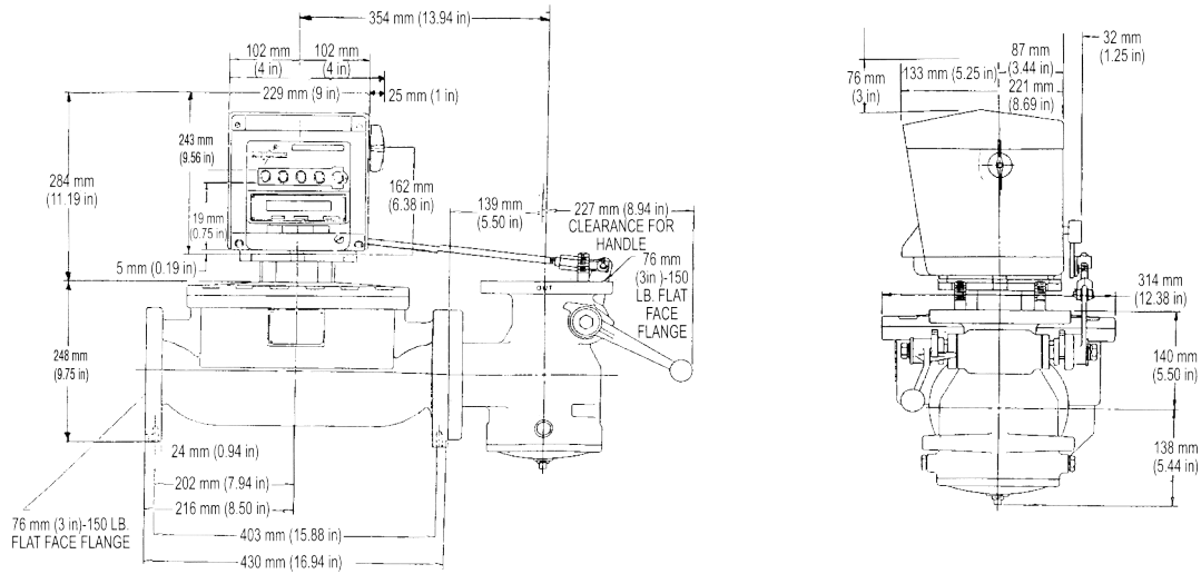
3" Type MP with 800 Series Register and Auto-Stop Valve
